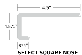
SELECT SQUARE NOSE
